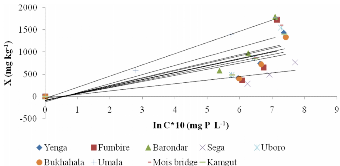
Fig. 4. Tempkin Equation for soils in the nine sites
