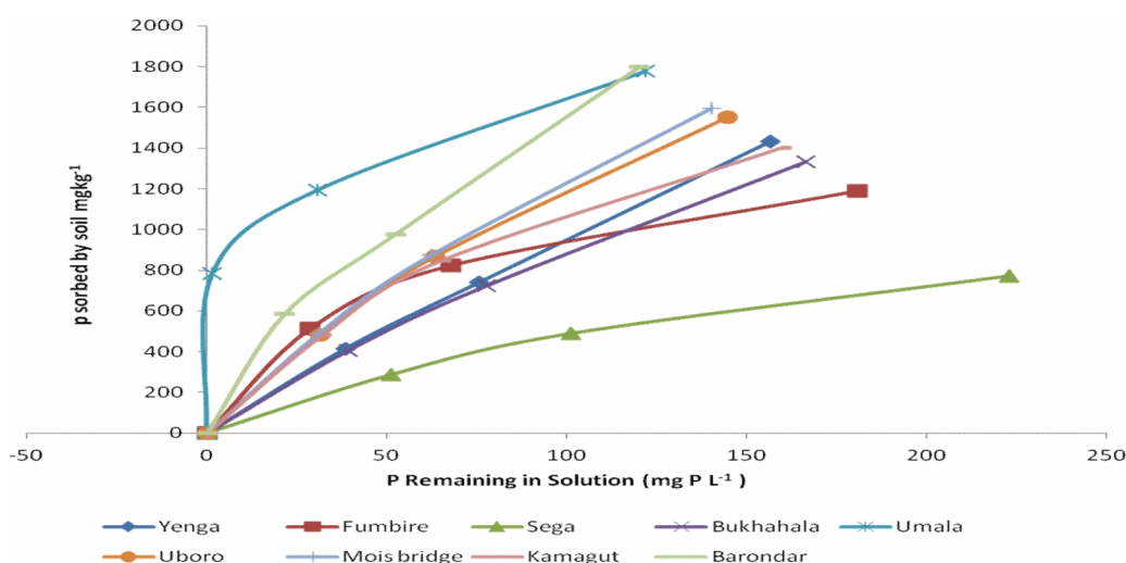
Fig. 1. Phosphate adsorption isotherm of soils from nine sites
