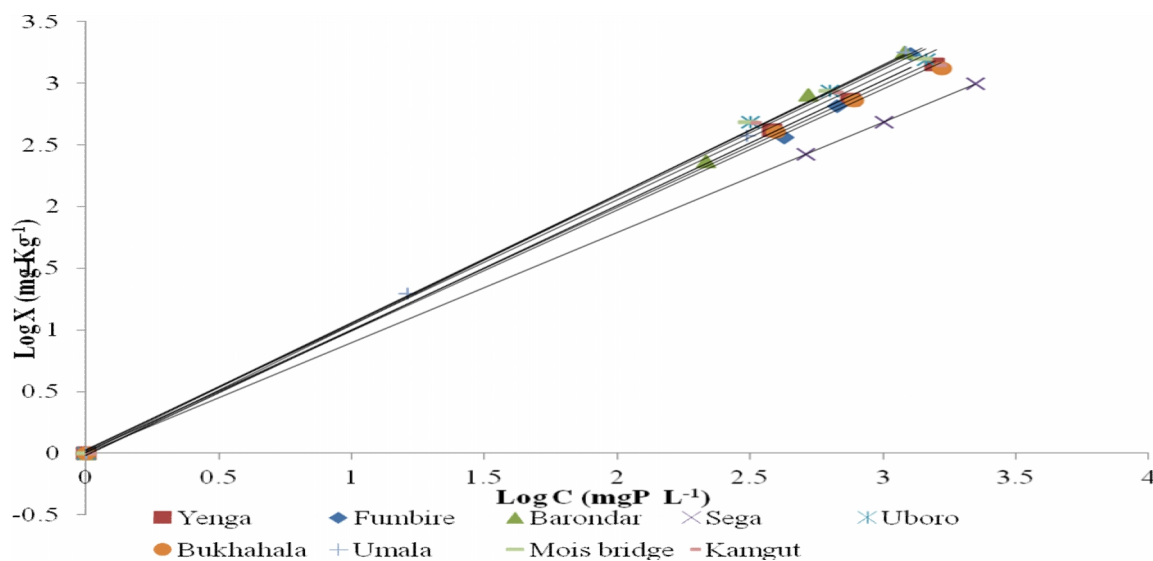
Fig. 3. Freundlich equation for soils in the nine sites
