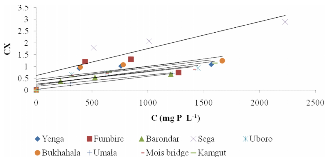
Fig. 2. Langmuir equation for soils in the nine sites
