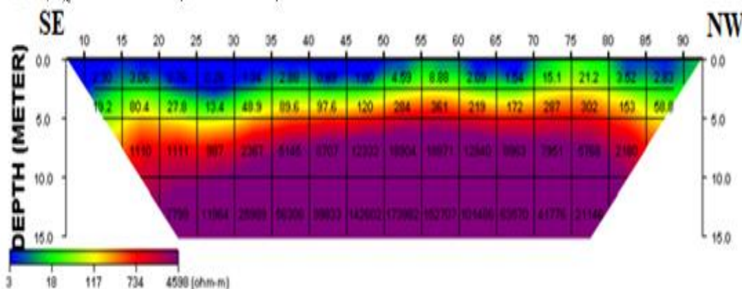
Fig. 11. 2D resistivity structure for Traverse 8
