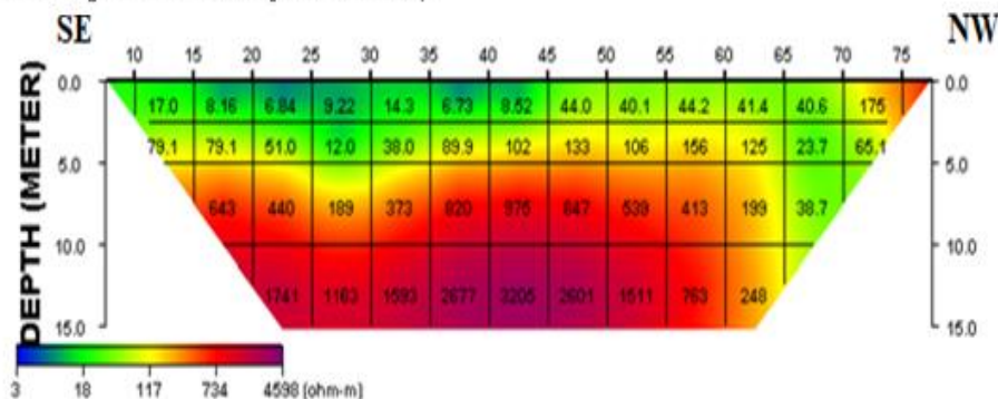
Fig. 7. 2D resistivity structure for Traverse 4
