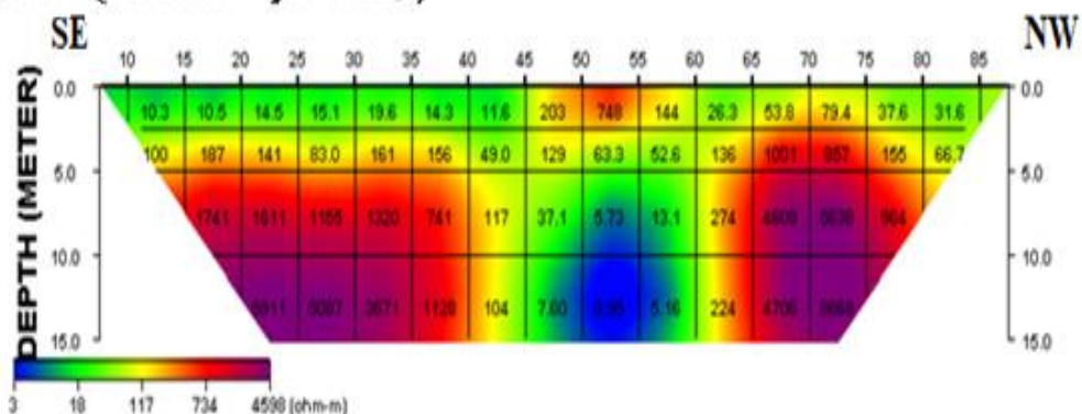
Traverse 6 (2-D Resistivity Structure)
