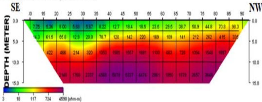
Traverse 5 (2-D Resistivity Structure)
