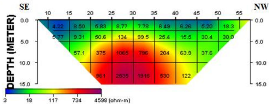
Fig. 6. 2D resistivity structure for Traverse 3
