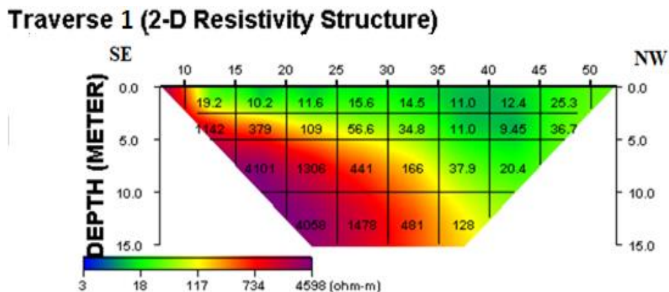
Fig. 4. 2D resistivity structure for Traverse 1
