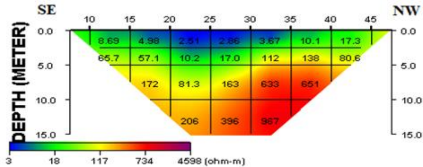
Fig. 5. 2D resistivity structure for Traverse 2
