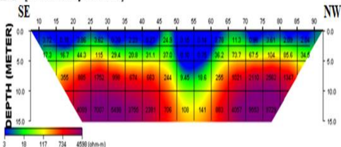
Fig. 10. 2D resistivity structure for Traverse 7
