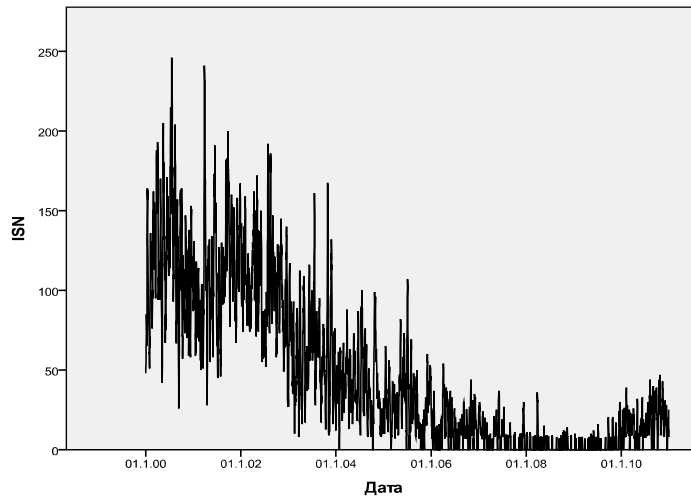
Fig. 1. Graphic demonstration of the SA in sunspot relative numbers (ISN) for the period 2000-2010
