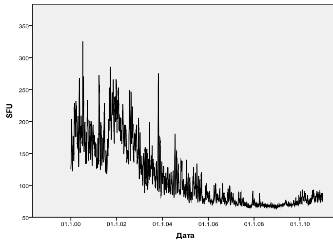
Fig. 2. Graphic demonstration of the SA in the values of the radio emission flux on the wave 10.7 cm (SFU) for the period 2000-2010
