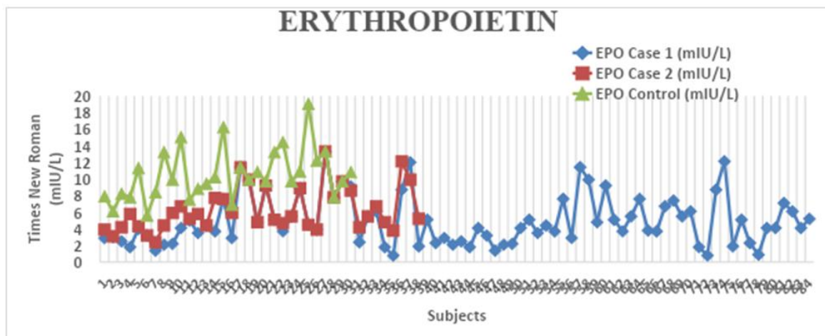
Fig. 1. Line Graph of erythropoietin levels of cases 1, 2 and control subjects
