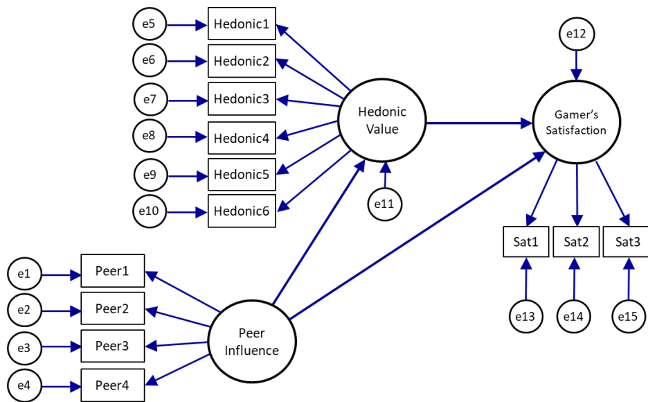
Fig. 2. Path diagram of the structured equation model
